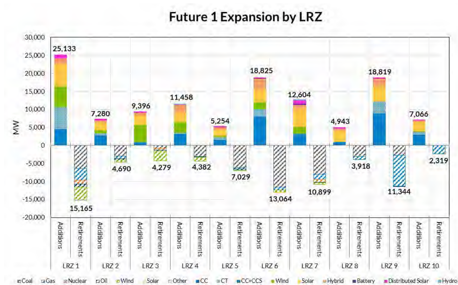
Figure 44: MISO Future 1 Resource Retirement and Addition Summary
