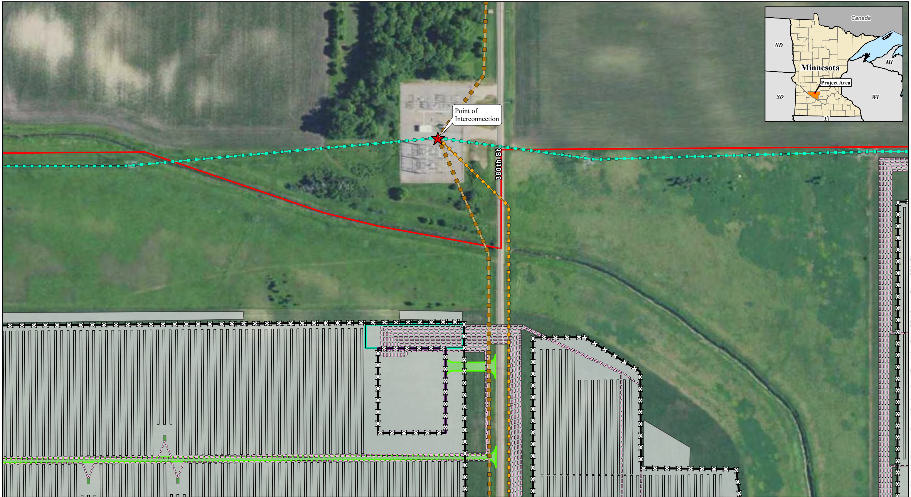
Figure 3 - Project Interconnect Facilities Gopher State Solar Project Ranger Power Renville County, Minnesota
