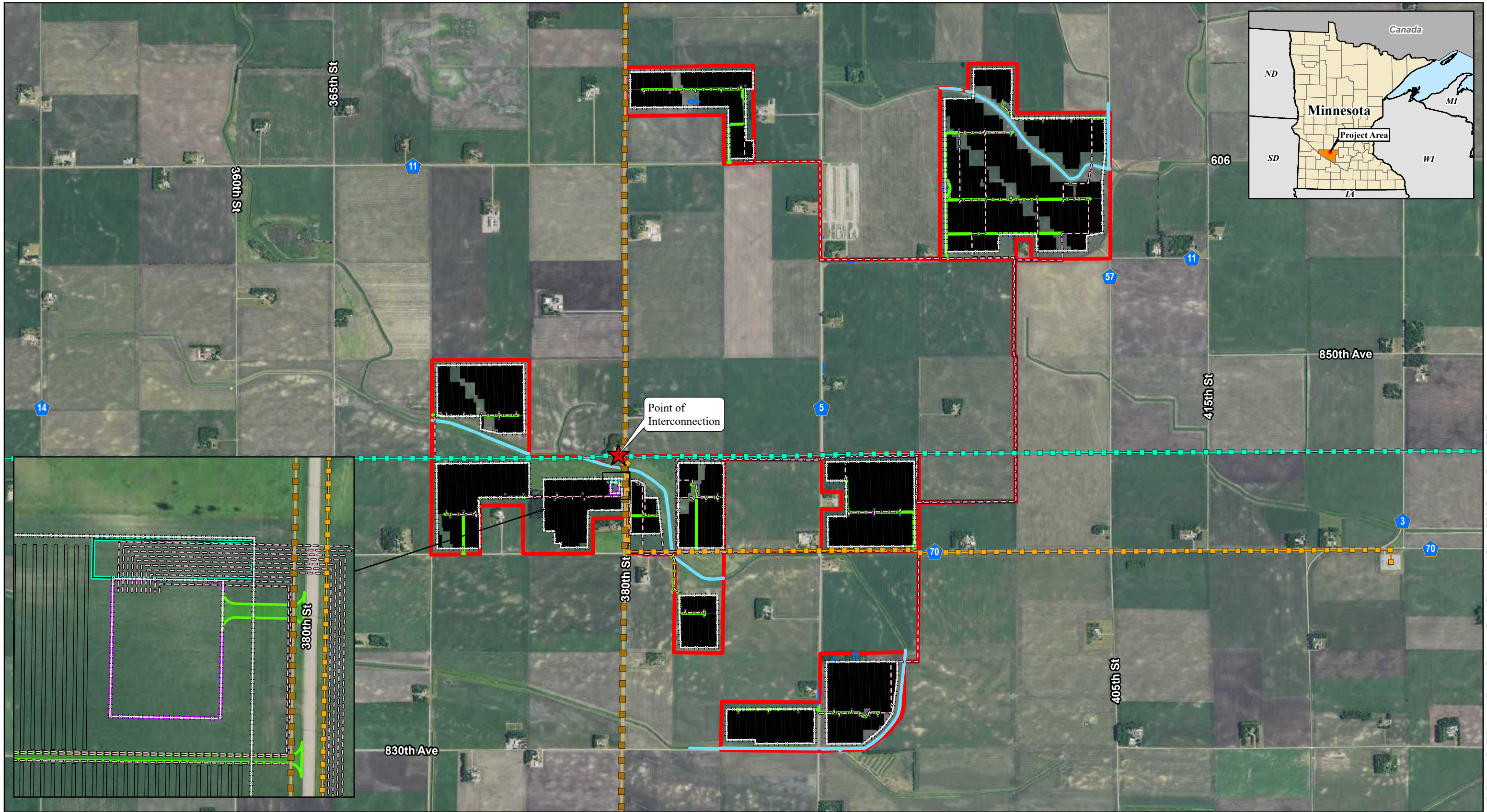
Figure 4 - Preliminary Facility Design Gopher State Solar Project Ranger Power Renville County, Minnesota
