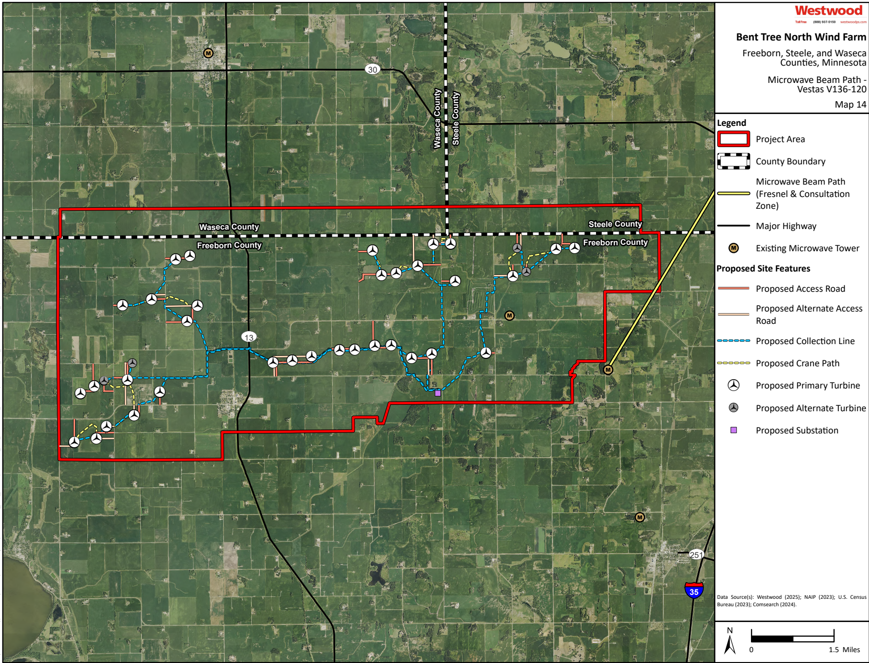
Map 14: Microwave Beam Oath - Vestas V136 - 120
