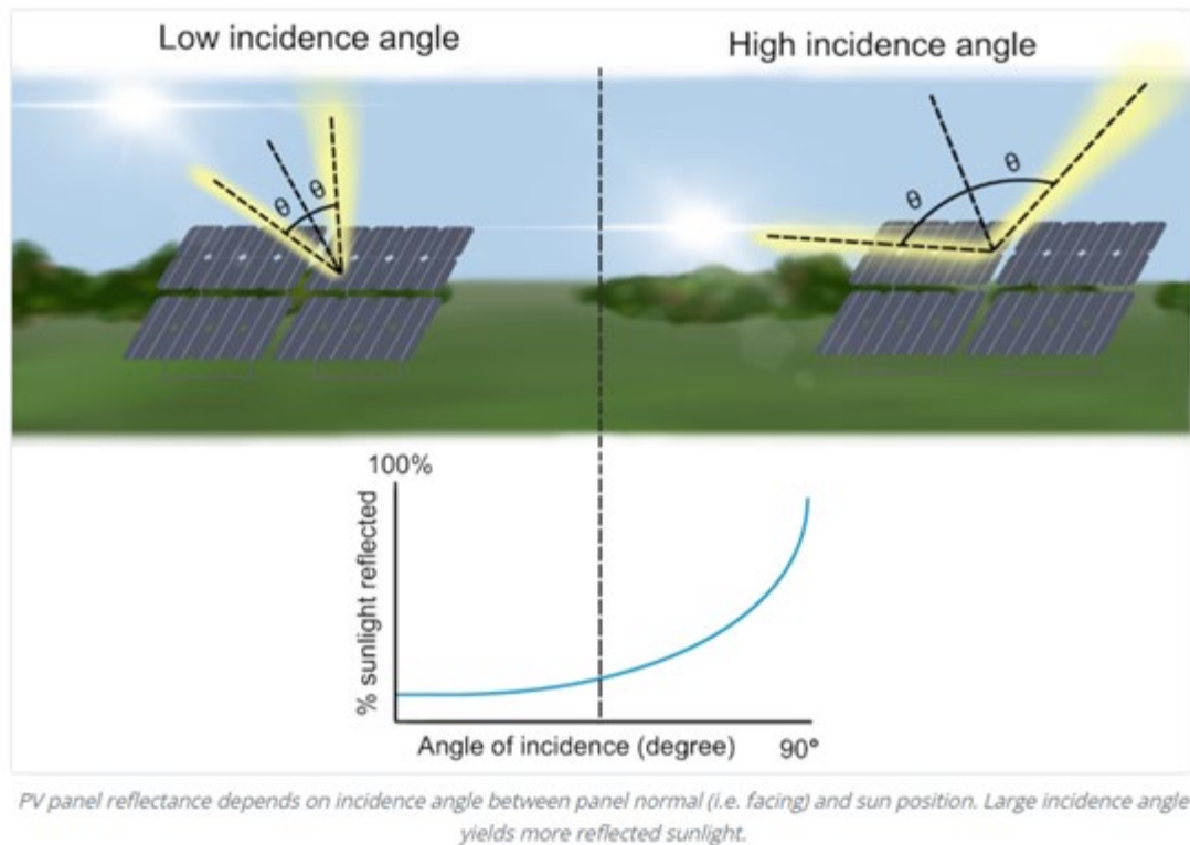
Figure 13: PV Panel Reflectance Diagram
