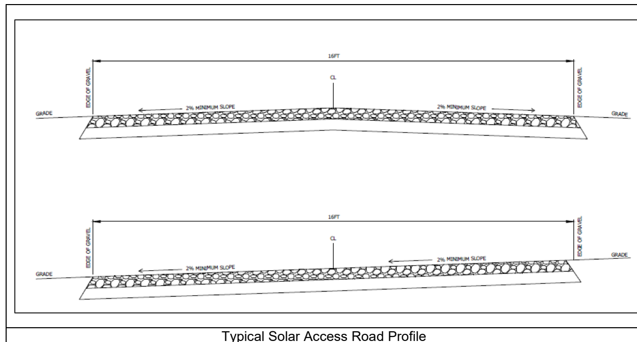
Figure 12: Typical Solar Access Road Profile
