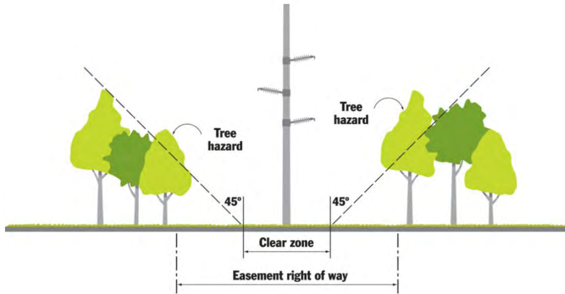
Figure 12-1: Wire/Border Zone
