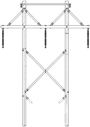
Typical H-Frame Structure
