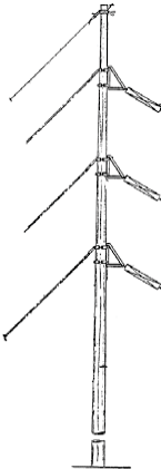
Typical Monopole Angle Structure
