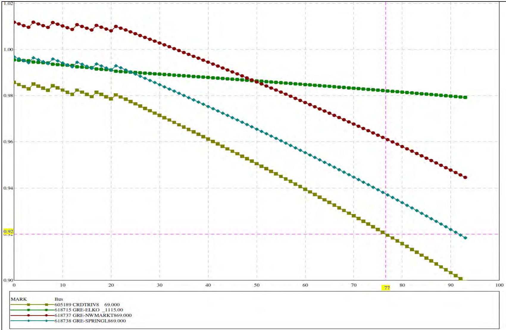
Figure F.3: Option 2(b)- Low voltage limit after 45 MW incremental load due to Credit River to Cleary Lake 69 kV line outage
