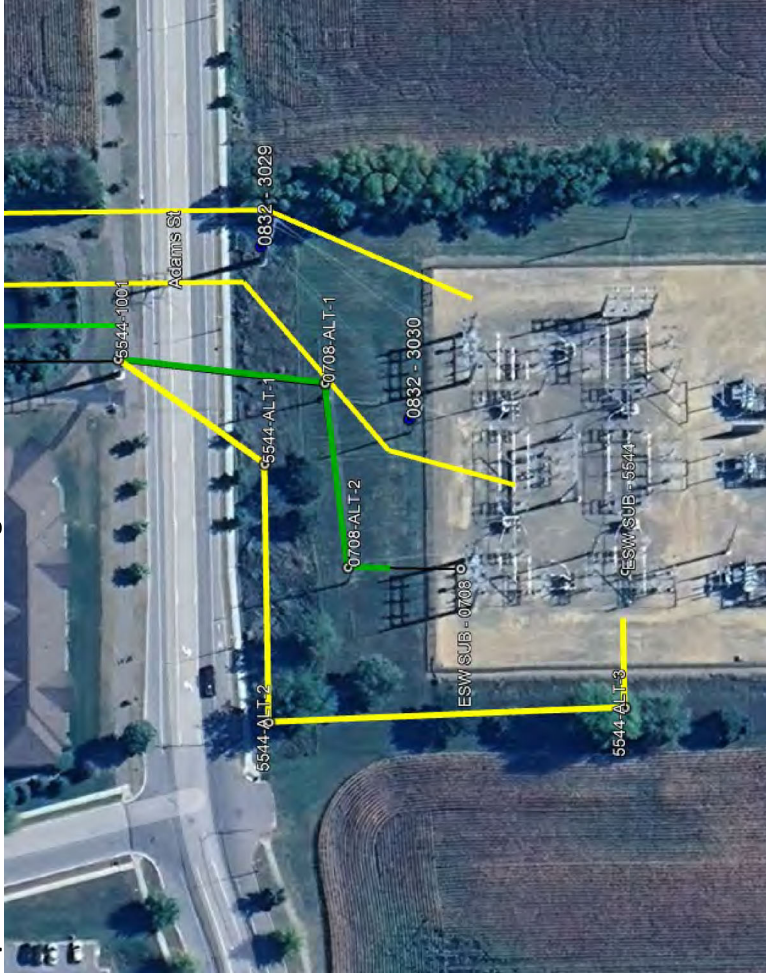
Option 1 South transmission reconfiguration at Eastwood Substation
