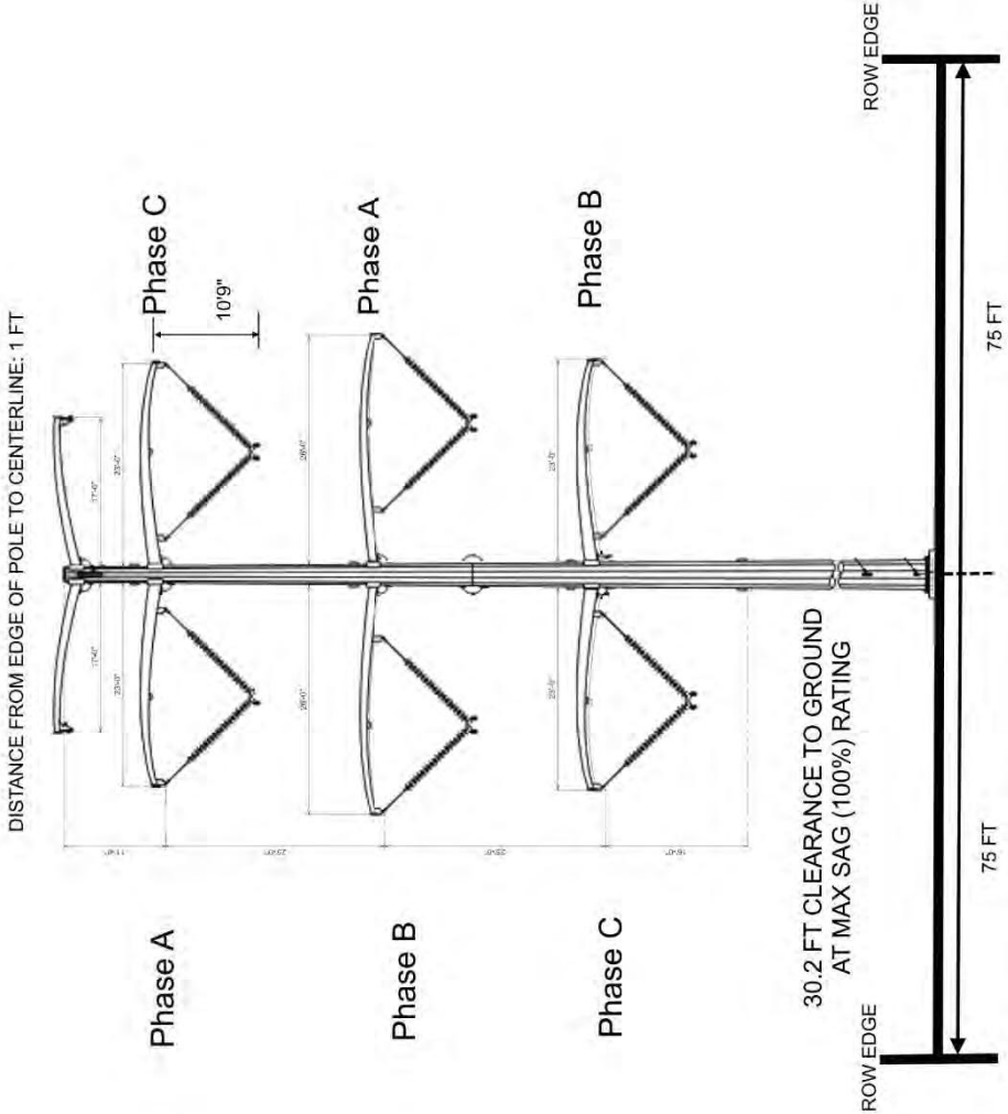
Figure 50: North Rochester – River 345 kV Double Circuit Line 965 345 kV
