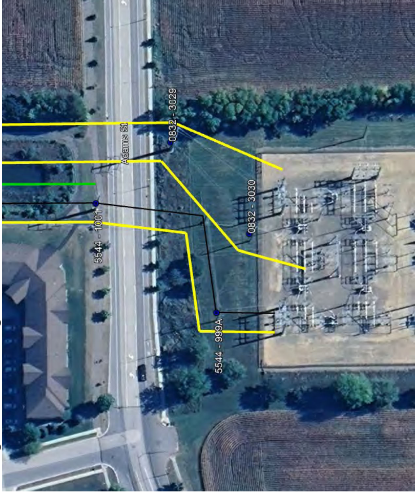
Existing transmission configuration at Eastwood Substation
