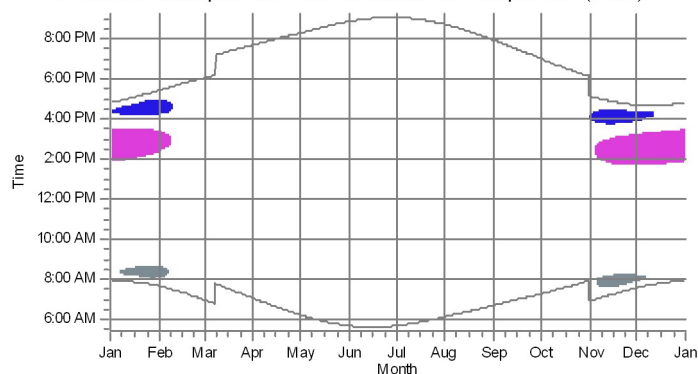
1: Shadow Receptor: 1.0 × 1.0 Azimuth: 0.0° Slope: 0.0° (1357)
