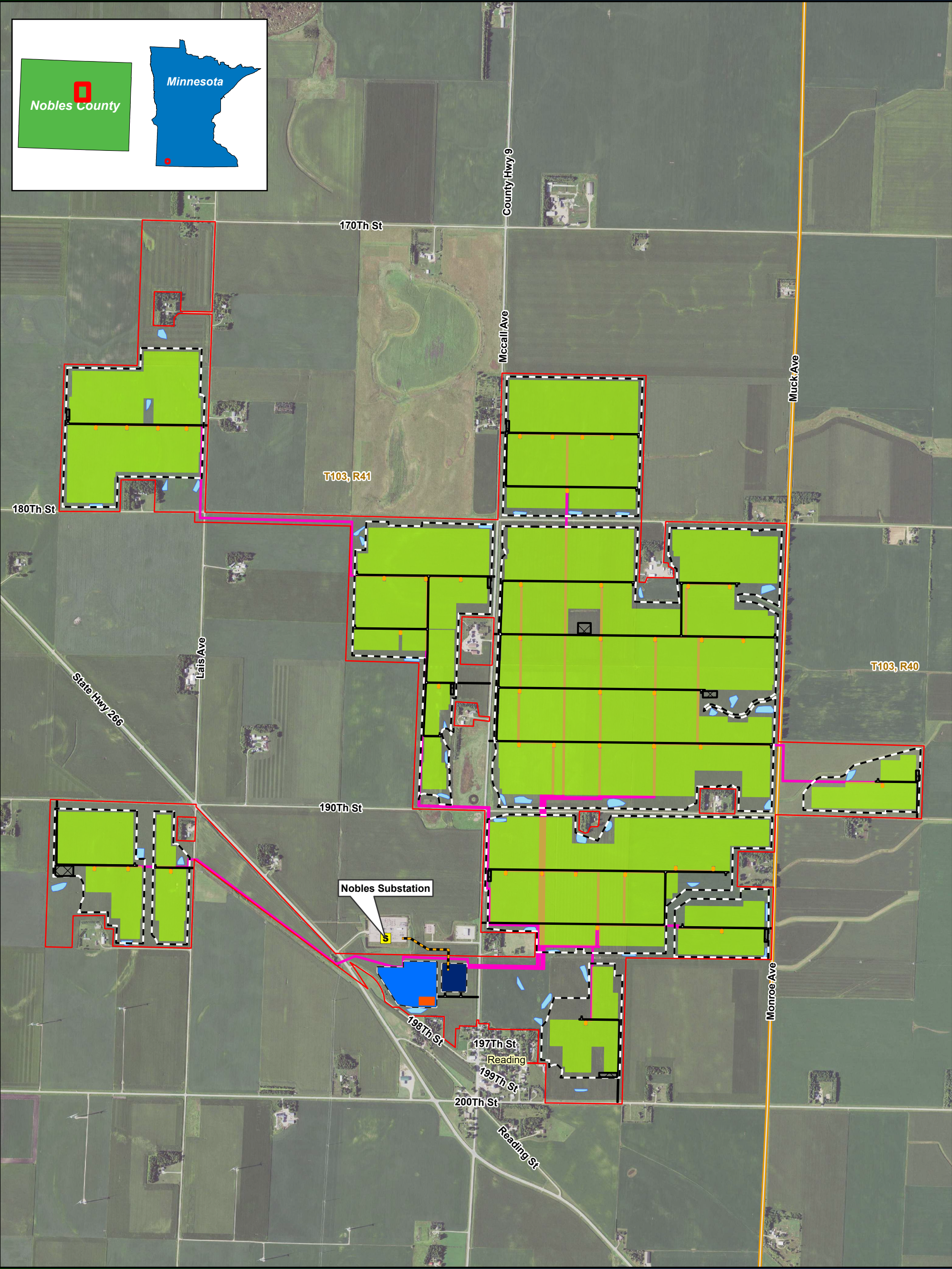
Figure 3 Preliminary Project Layout Summit Lake Solar and BESS Projects Nobles County, MN
