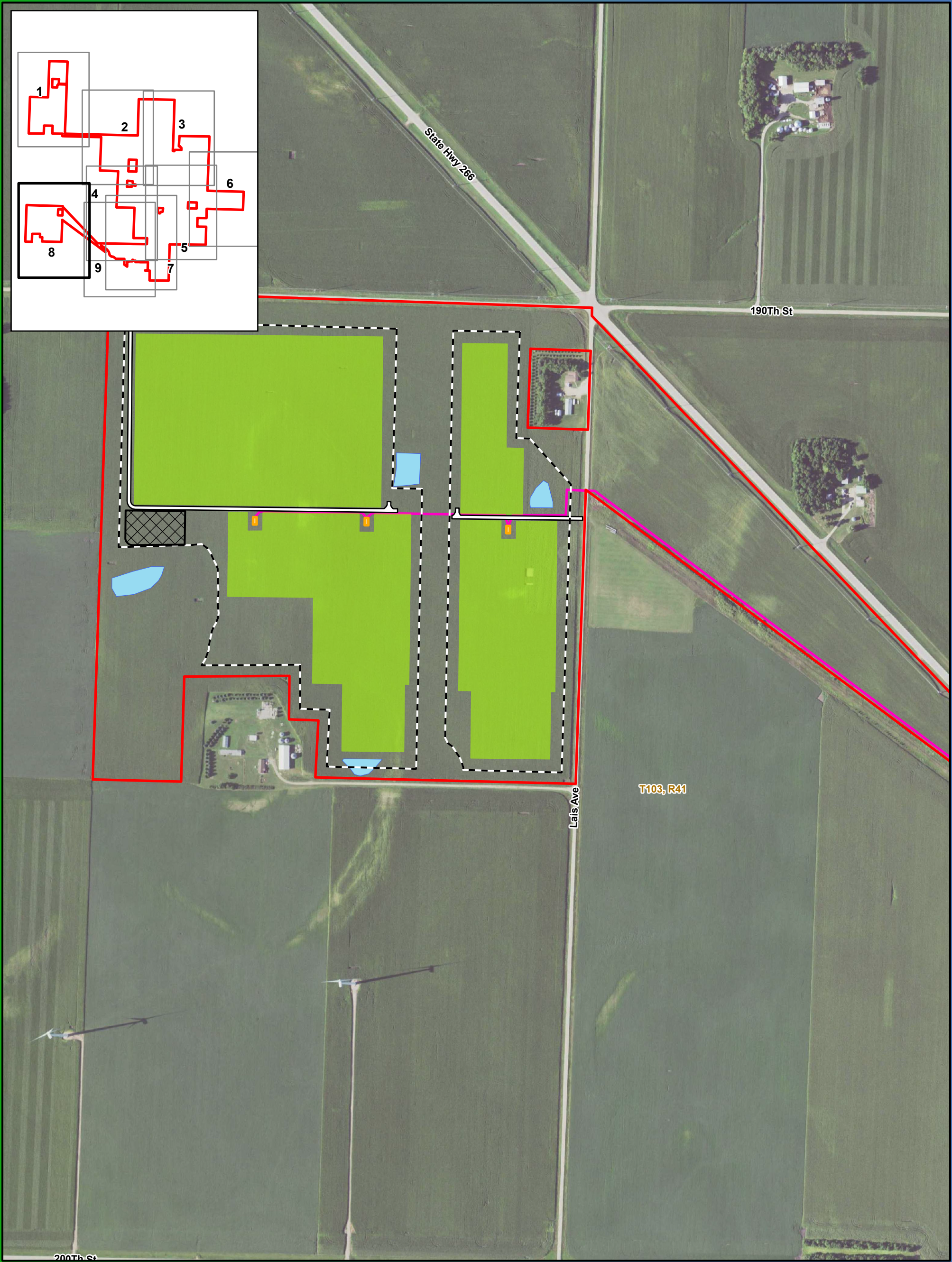
Figure 4 Detailed Preliminary Project Layout Summit Lake Solar and BESS Projects Nobles County, MN
