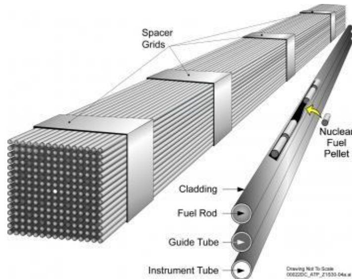
Figure I. Example of a Nuclear Fuel Assembly
