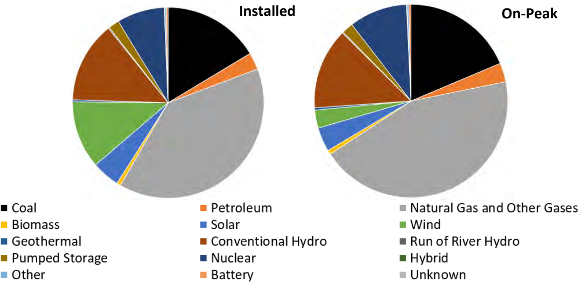
Figure 11: 2022 BPS Generation Capacity by Fuel Type
