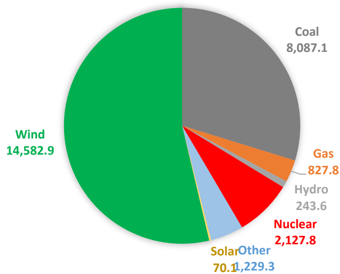
MISO NORTH FUEL MIX (MW) NOV 28 7 AM
