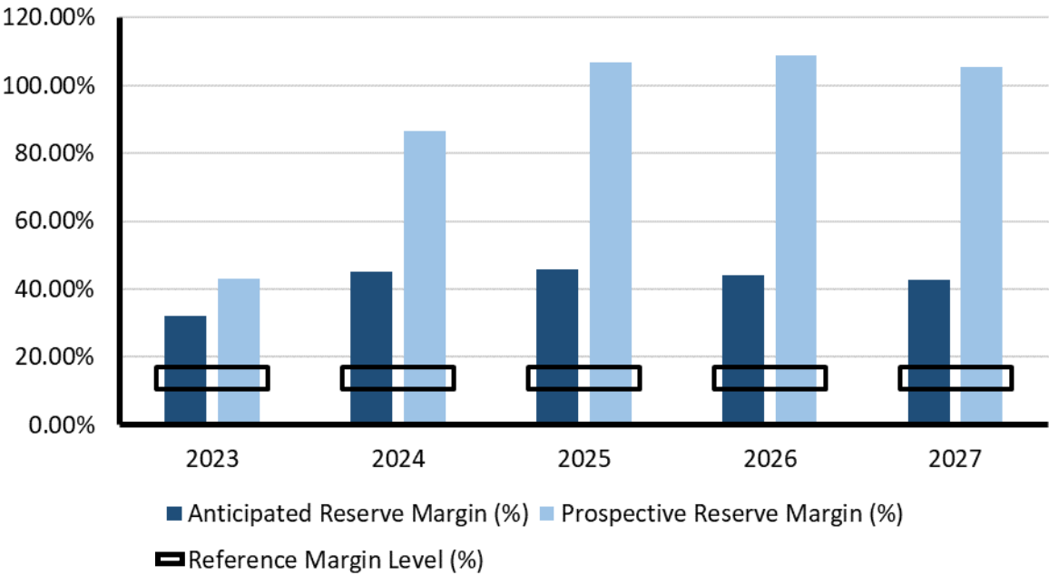
Figure 9: Texas RE-ERCOT Five-Year Projected Reserves (ARM and PRM)
