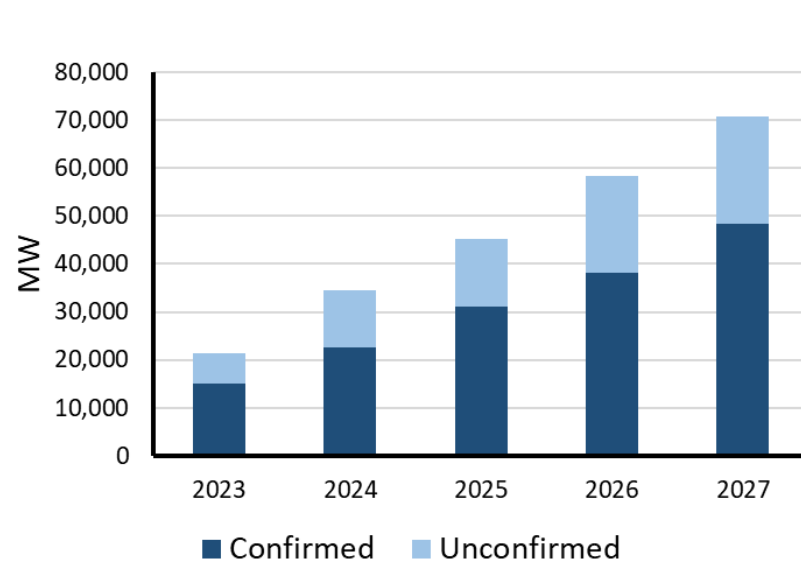
Figure 16: Projected Generation Retirement Capacity Through 2027
