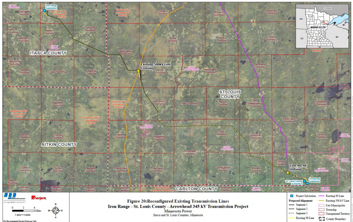
Figure 20. Reconfigured Existing Transmission Lines
