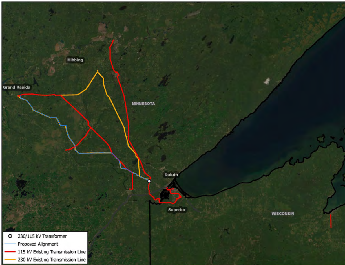
Figure 25. Existing Transmission Lines Included in the Upgrade Alternative
