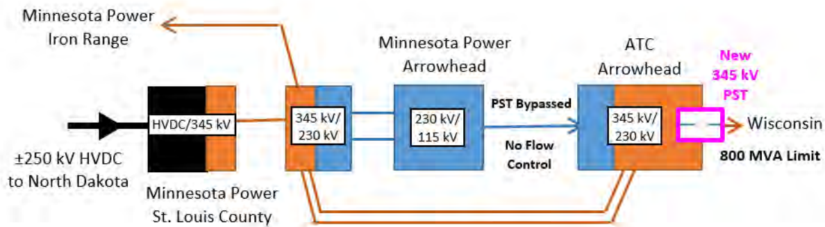
Figure 28. Alternative Configuration, Install 345 kV PST
