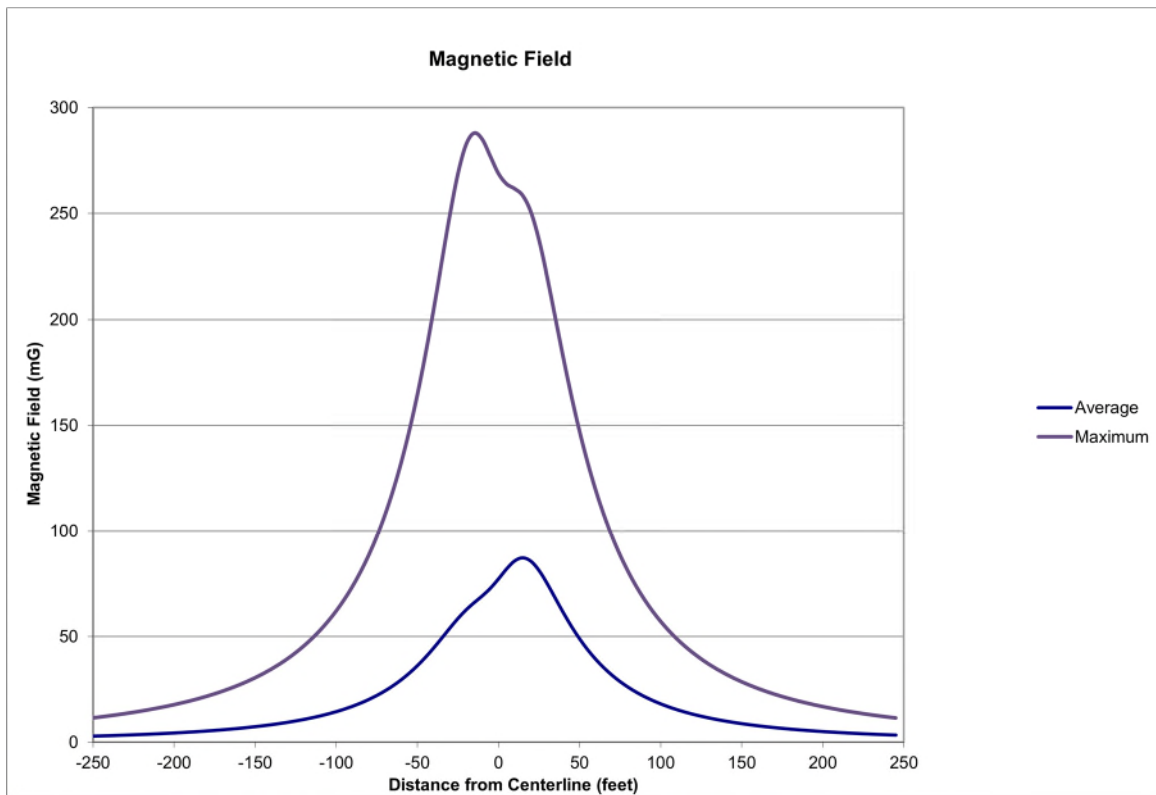
Figure S-17 Calculated Magnetic Flux density (mG) for proposed Single Pole, Tangent/Davit Arm, 345 kV Double Circuit - Wilmarth – North Rochester 345 kV & Line 964 345 kV
