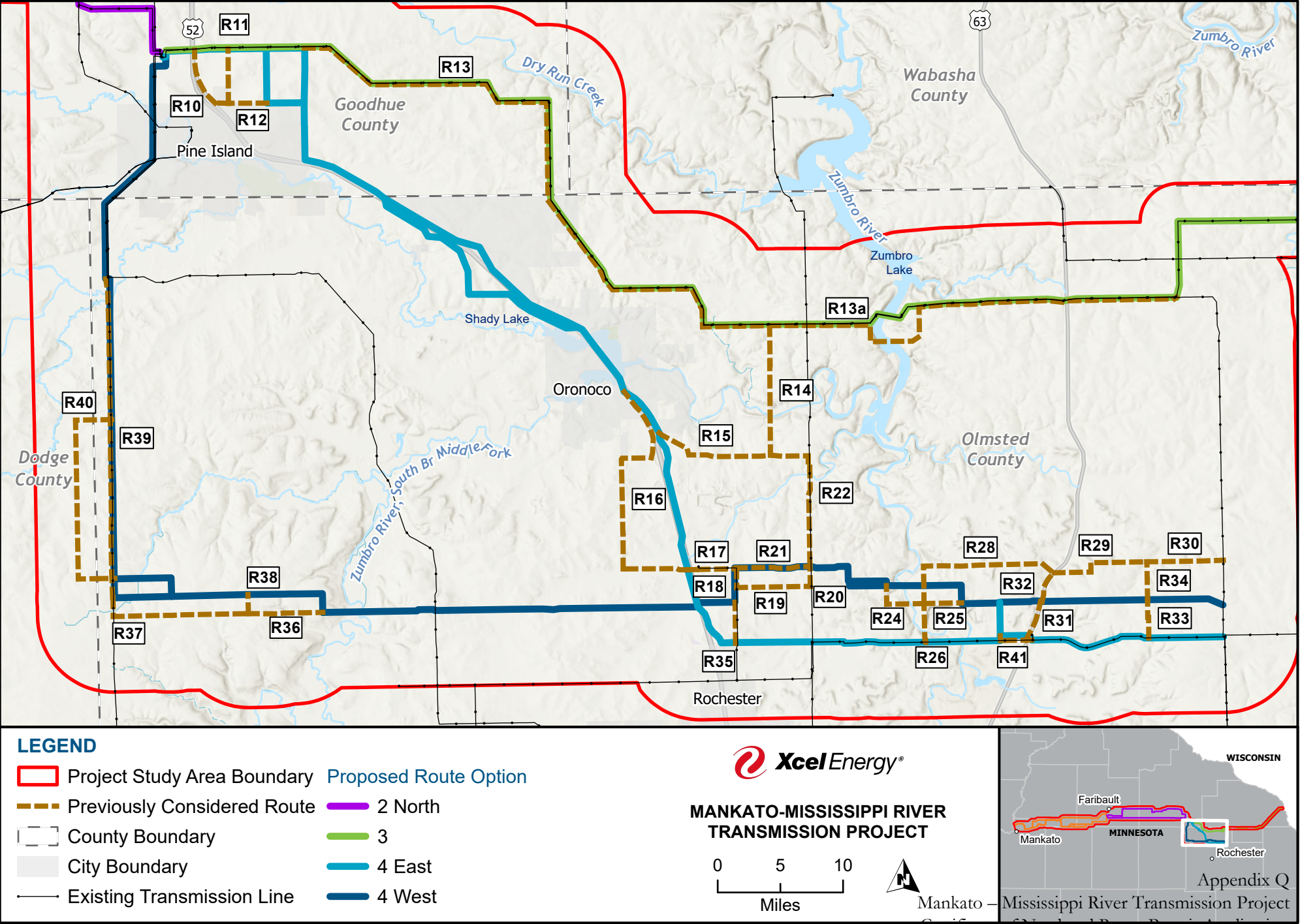
FIGURE Q-5 SEGMENT 4: PREVIOUSLY CONSIDERED ROUTES
