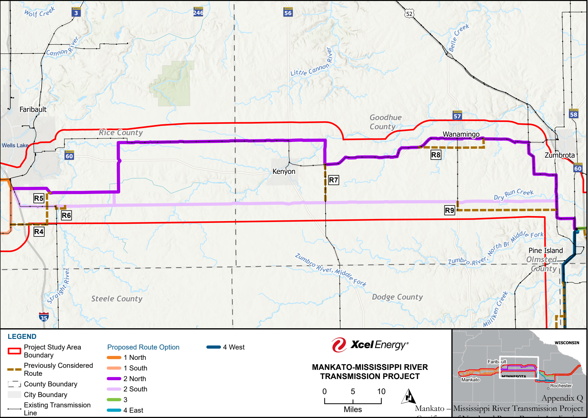
FIGURE Q-3 SEGMENT 2: PREVIOUSLY CONSIDERED ROUTES
