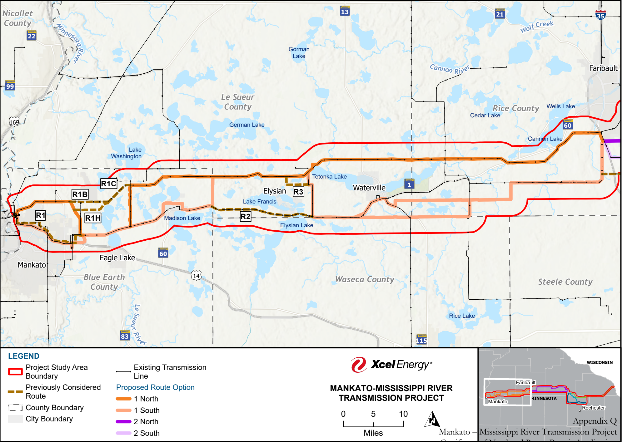
FIGURE Q-1 SEGMENT 1: PREVIOUSLY CONSIDERED ROUTES
