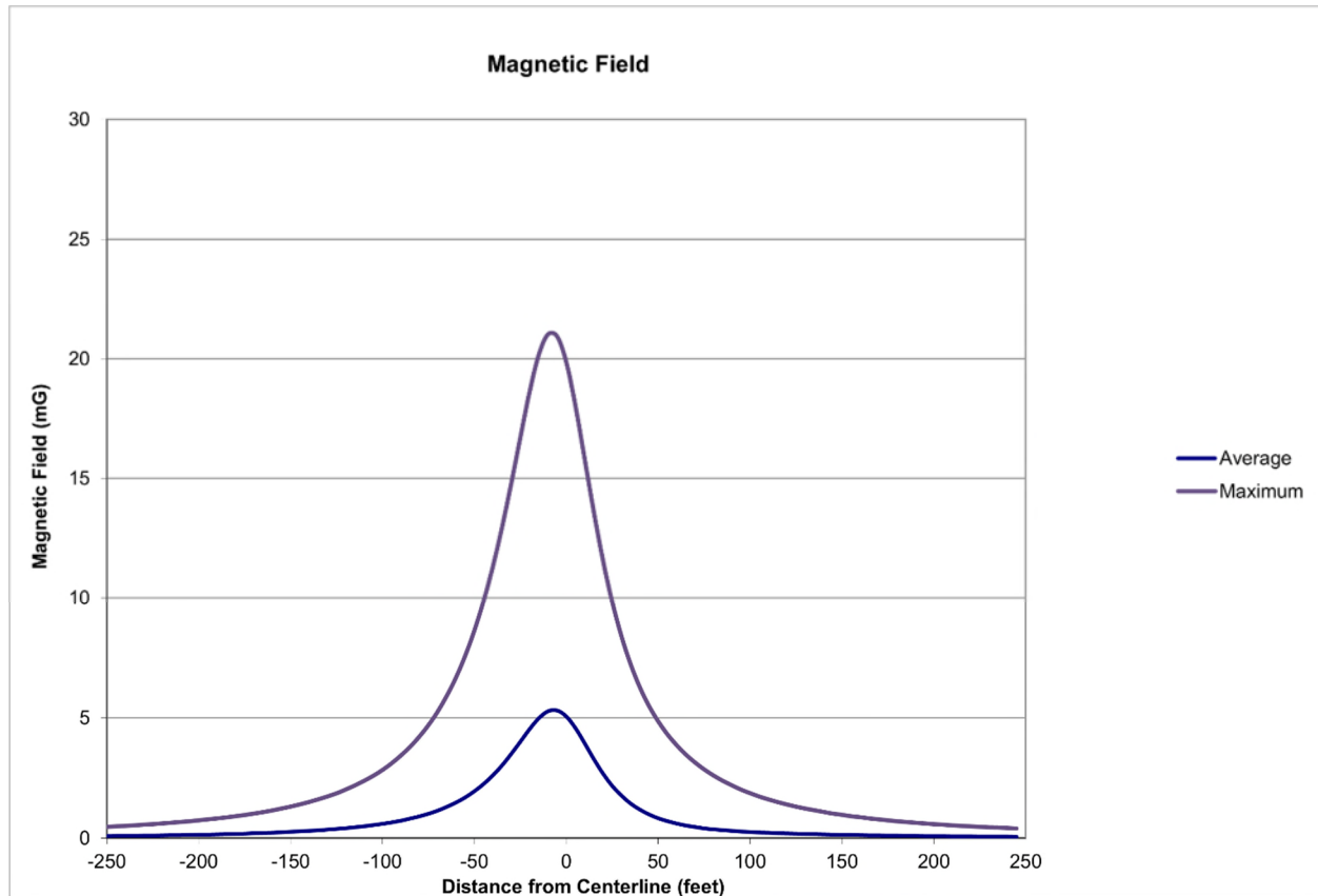
Figure S-19 Calculated Magnetic Flux density (mG) for proposed Single Pole, Davit, 161/69 kV Double Circuit - North Rochester – Chester 161 kV & Peoples Line 69 kV
