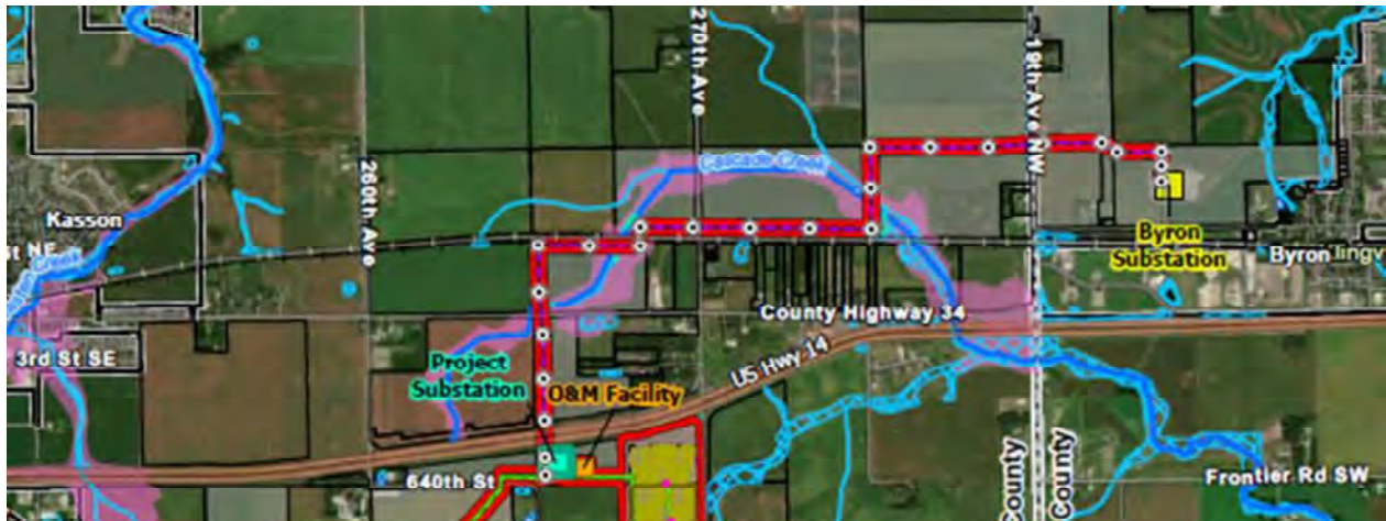
Figure 2. HVTL proposed route map.
