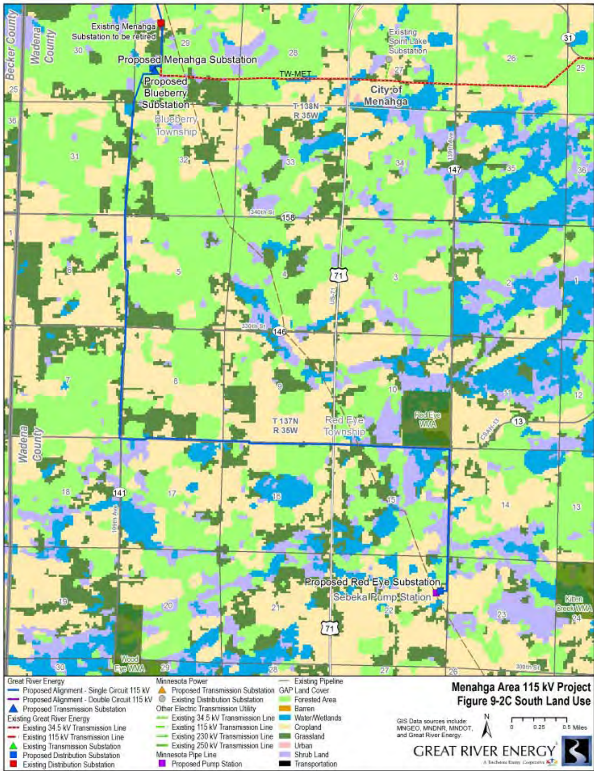
Figure 9-2C. Land Use-South
