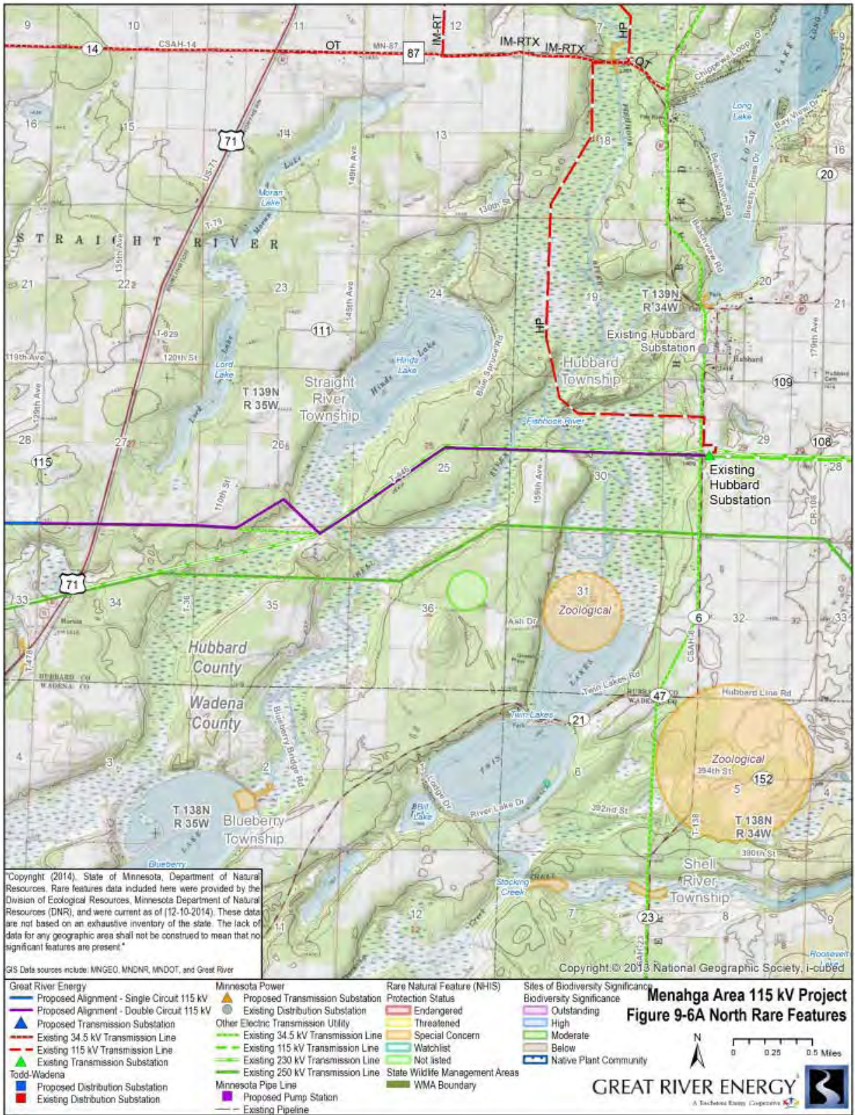
Figure 9-6A. Rare Features-North
