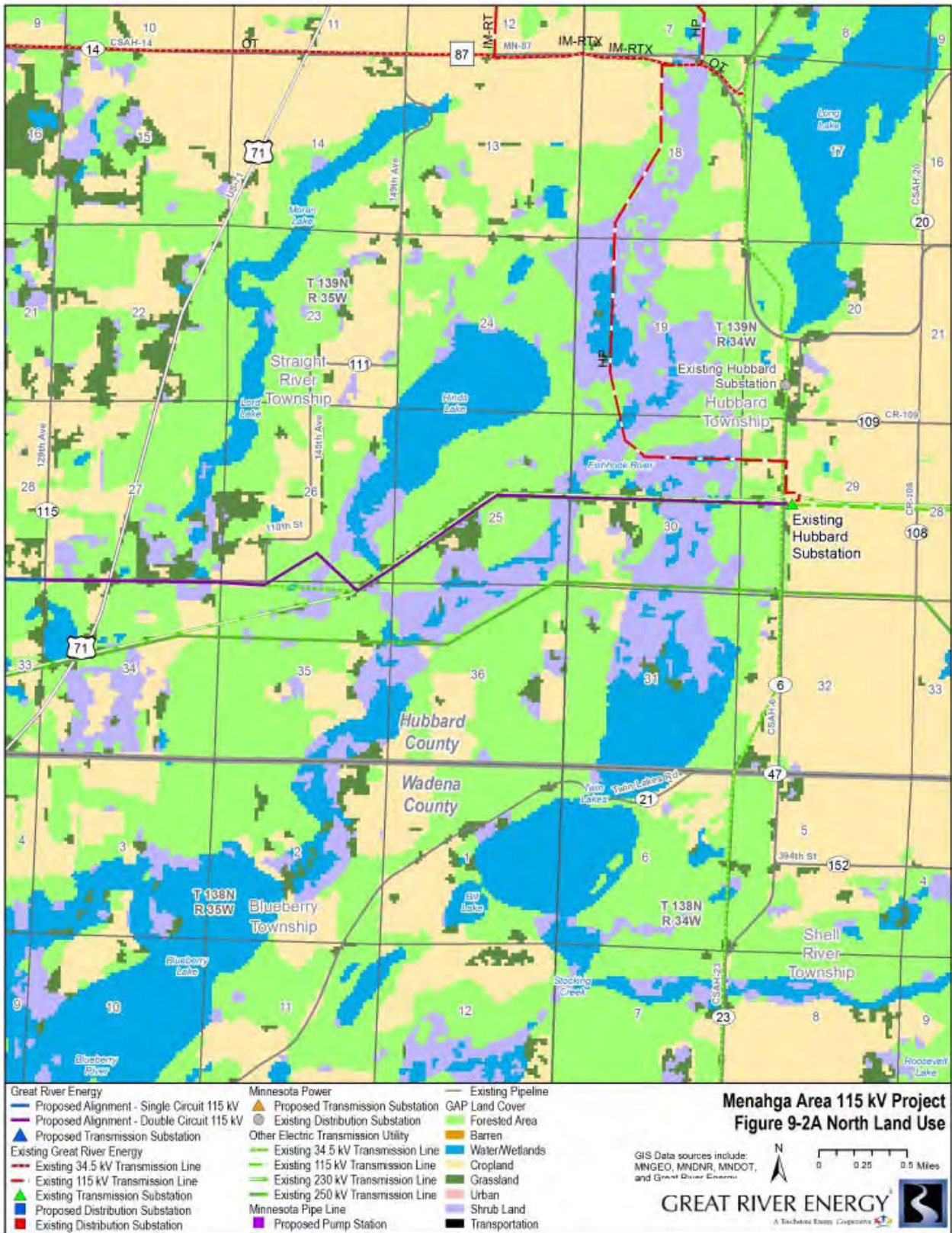
Figure 9-2A. Land Use-North
