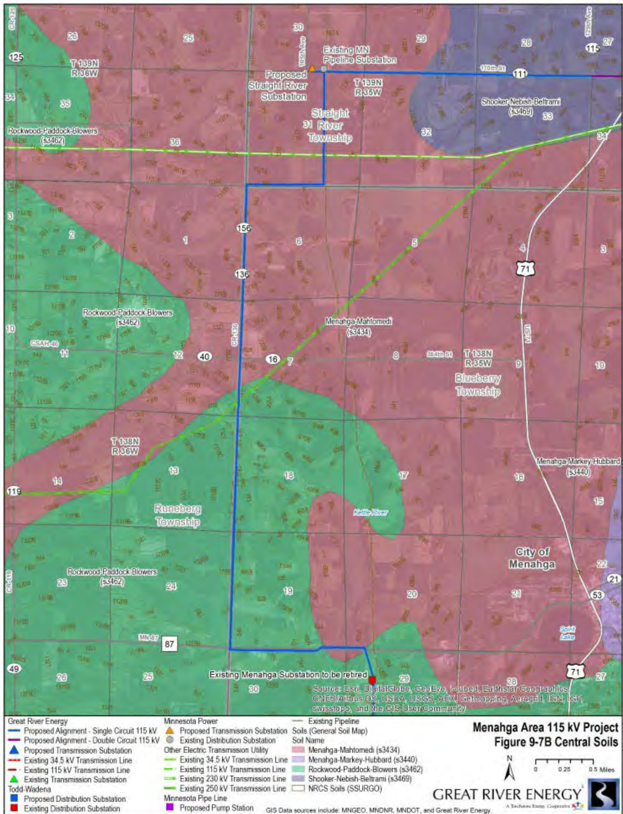
Figure 9-7B. Soils-Central
