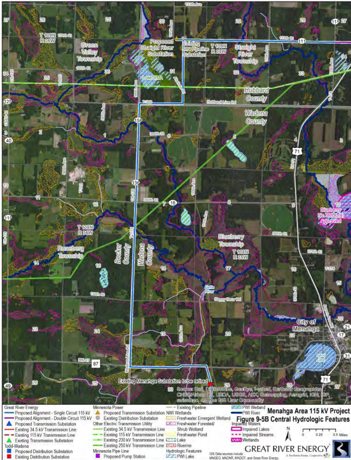
Figure 9-5B. Hydrologic Features-Central
