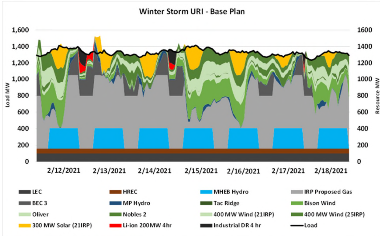
Figure 13. Energy Supply Performance During Winter Storm Uri with Base Plan 13
