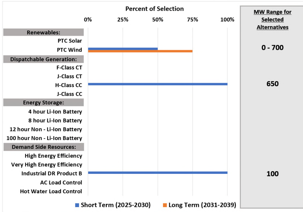
Figure 27. Full Biomass/Gas Refuel Capacity Expansion Results +500 MW Growth Scenario
