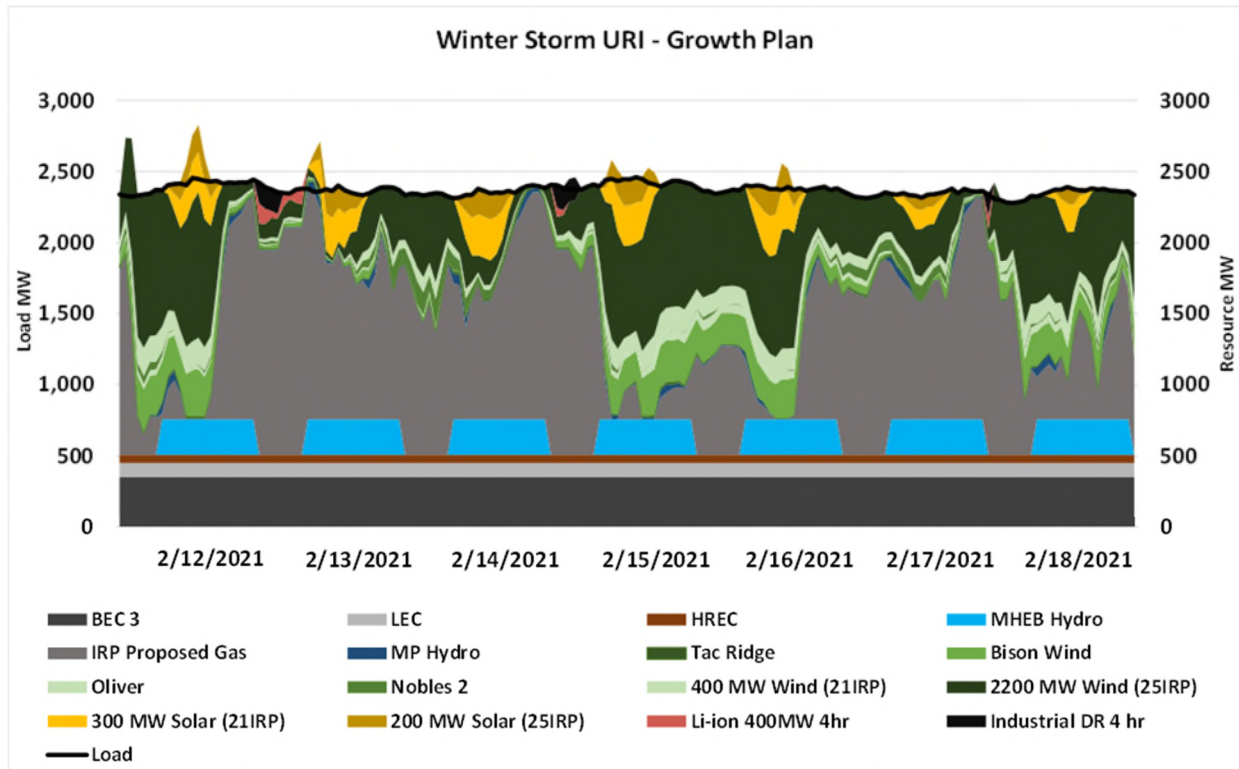
Figure 14. Energy Supply Performance During Winter Storm Uri with Growth Plan 14
