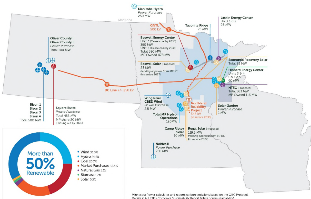
Figure 7: Minnesota Power's Current and Proposed Generation Supply 4,5
