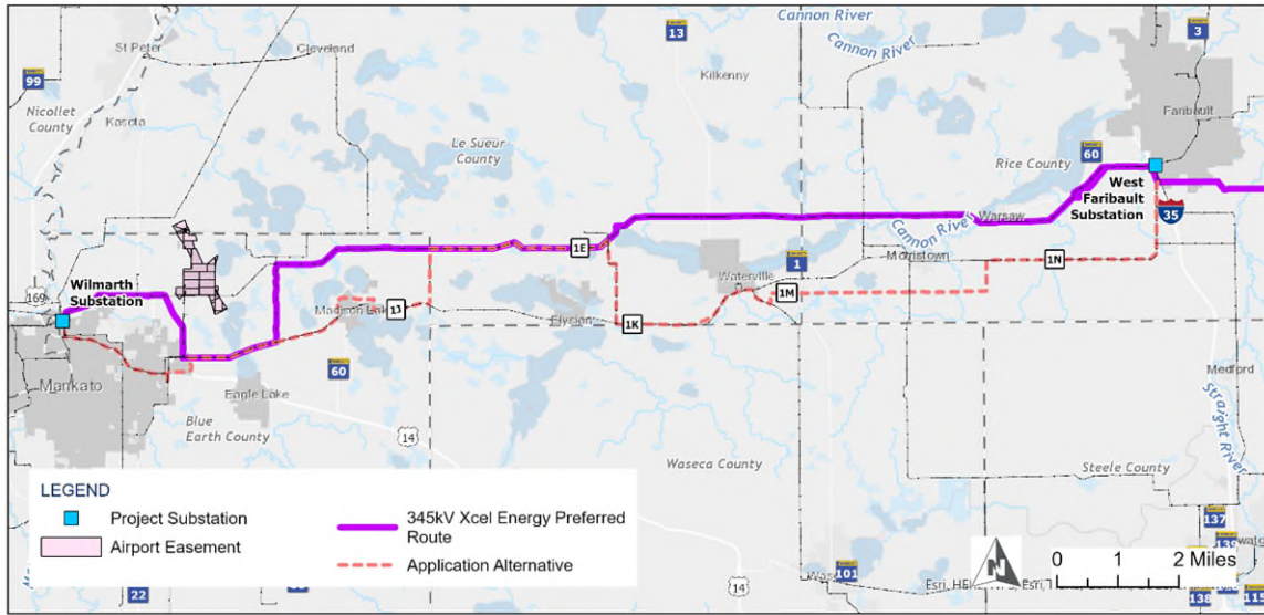
Figure 4. Xcel Energy's Preferred Route for Segment 1
