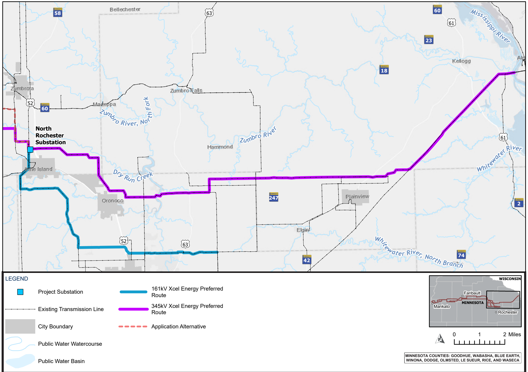
FIGURE 5 XCEL ENERGY PREFERRED ROUTE: SEGMENT 3
