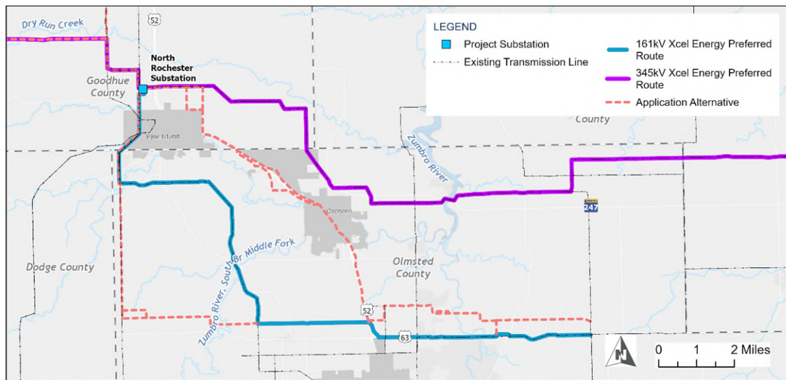
Figure 7. Xcel Energy's Preferred Route for Segment 4
