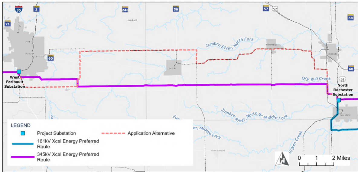
Figure 5. Xcel Energy's Preferred Route for Segment 2
