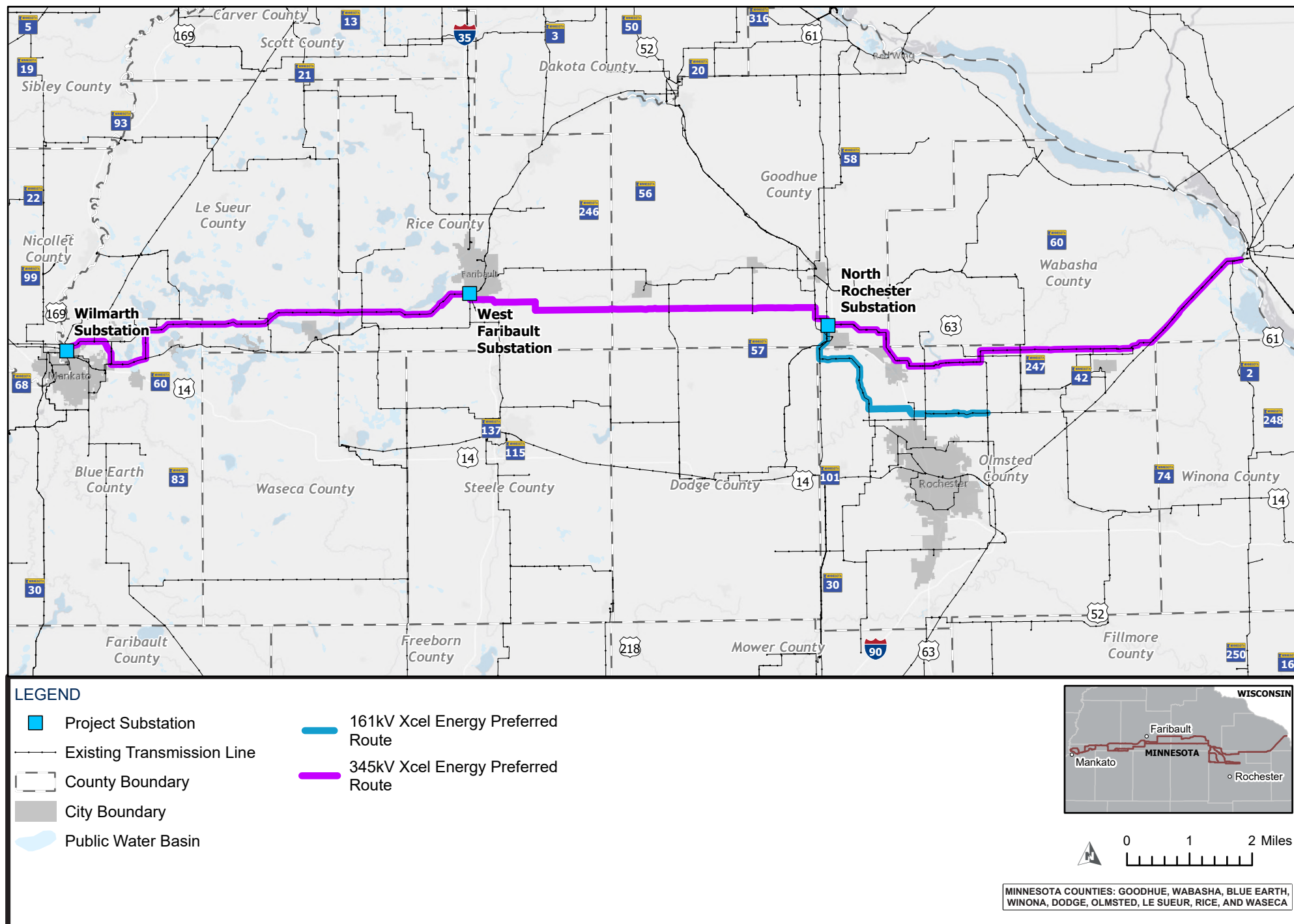
FIGURE 2 XCEL ENERGY PREFERRED ROUTE
