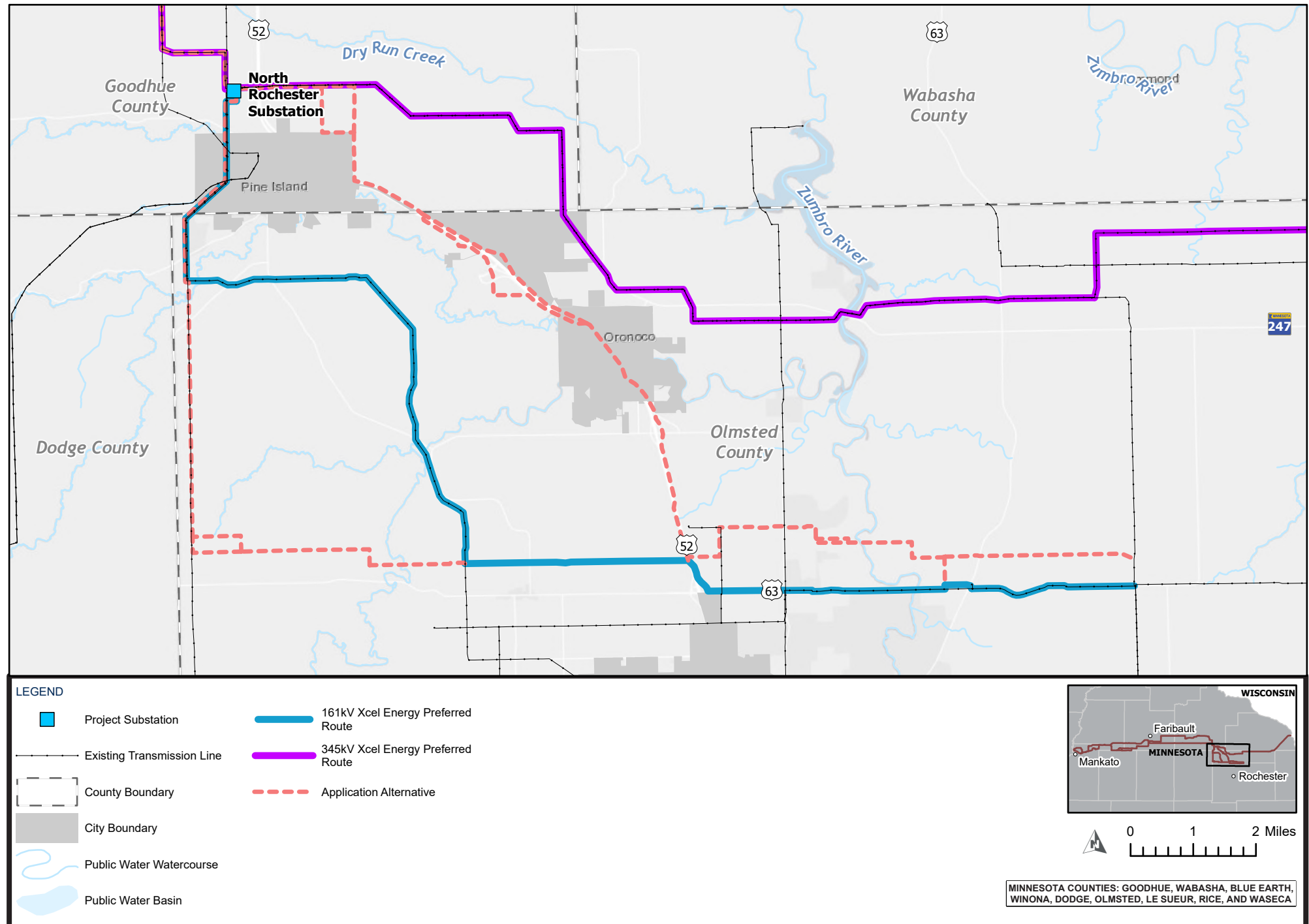
FIGURE 6 XCEL ENERGY PREFERRED ROUTE: SEGMENT 4
