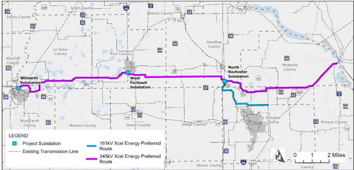
Figure 3. Xcel Energy's Preferred Route
