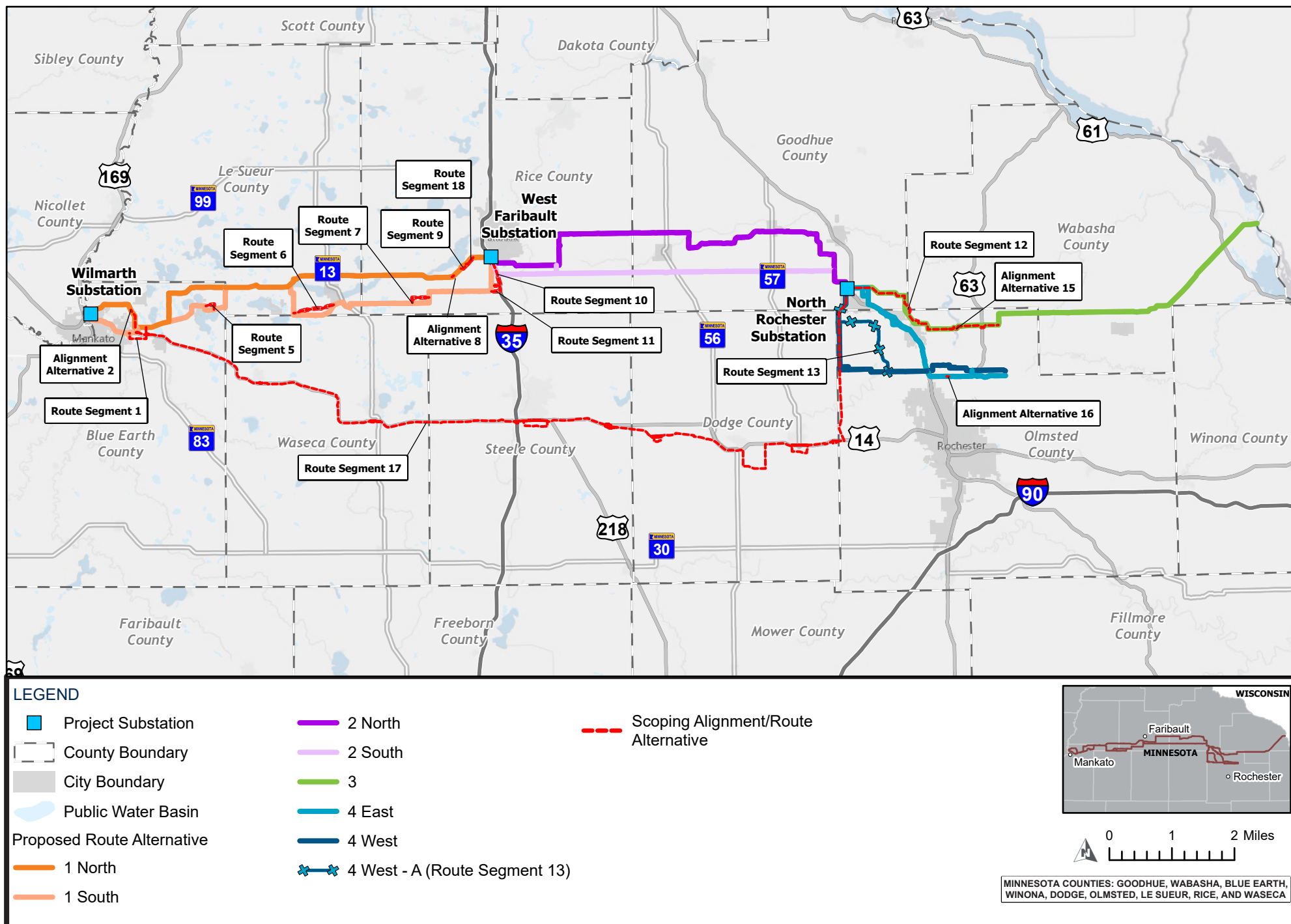
FIGURE 1 ALL PROPOSED ROUTES
