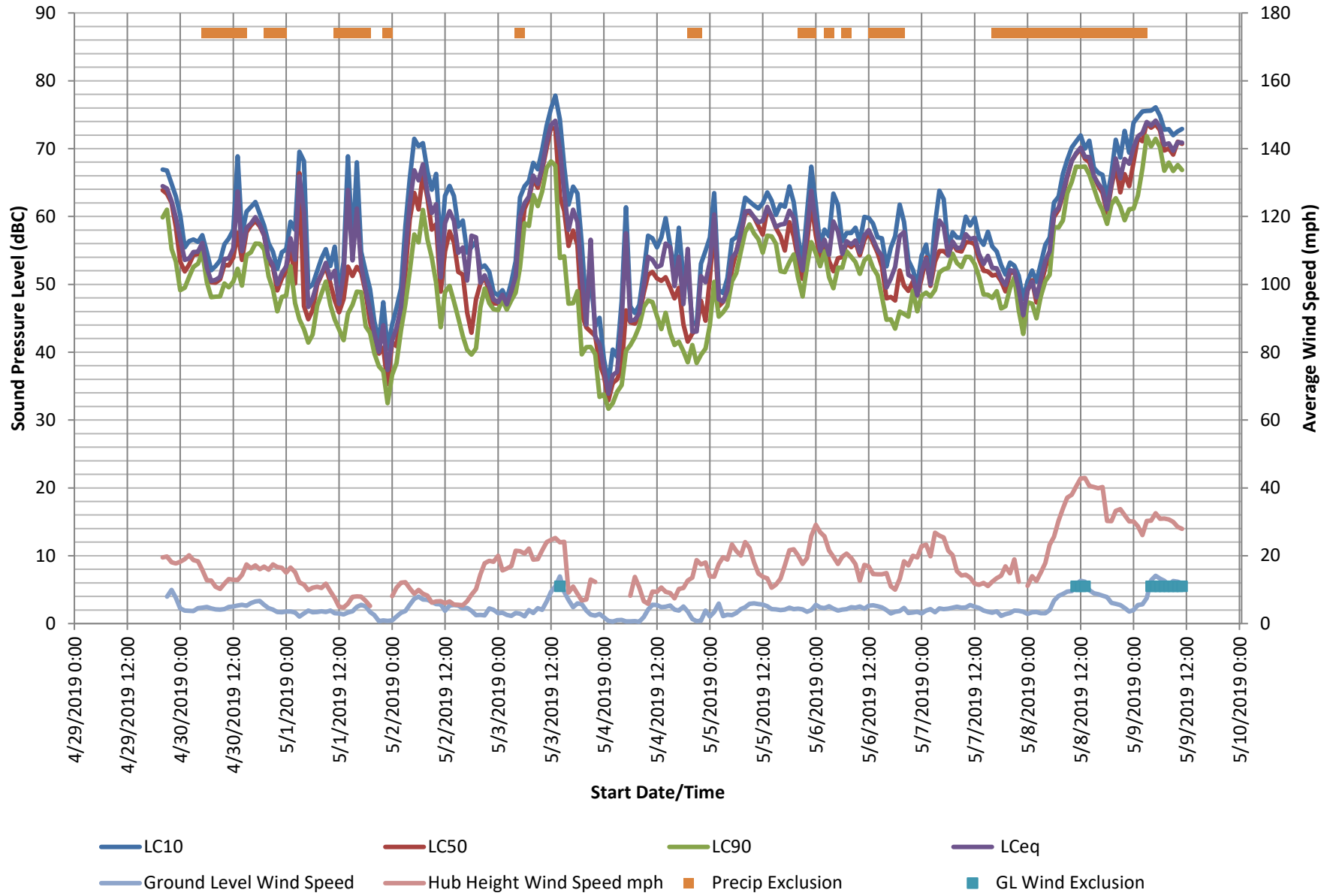
Figure 5-15: Measured/Calculated Hourly C-weighted Sound Pressure Levels (dBC) versus Meteorological Data Location 4
