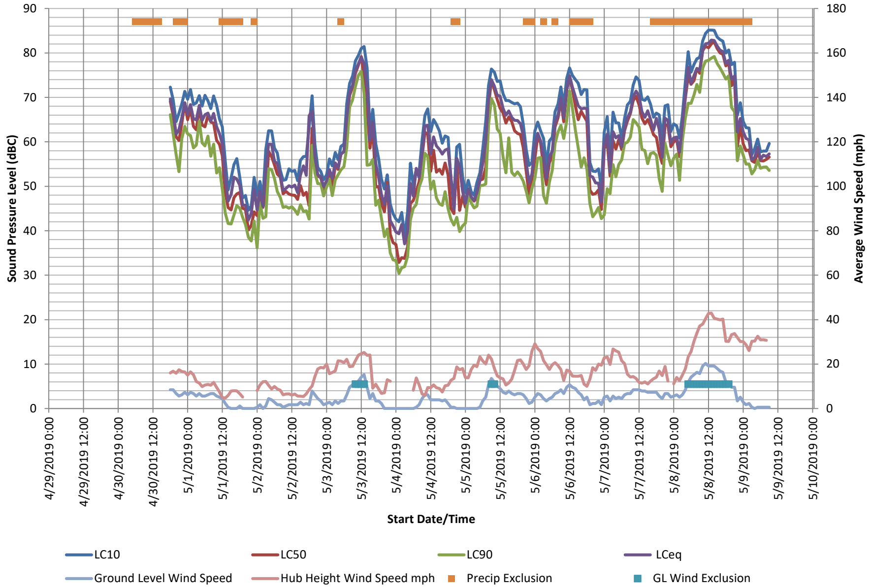
Figure 5-11: Measured/Calculated Hourly C-weighted Sound Pressure Levels (dBC) versus Meteorological Data Location 2
