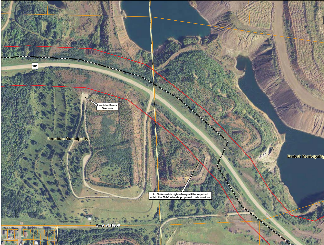
FIGURE 5 Proposed HVTL Route
