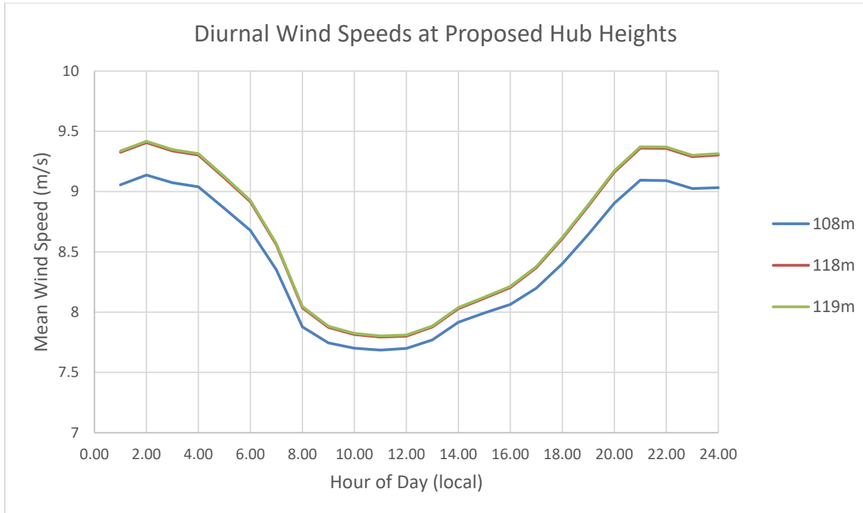
Chart 9.1-1: Diurnal Wind Speeds
