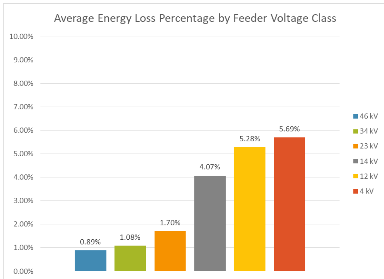
Figure 2: Average Energy Loss Percentage by Feeder Voltage Class
