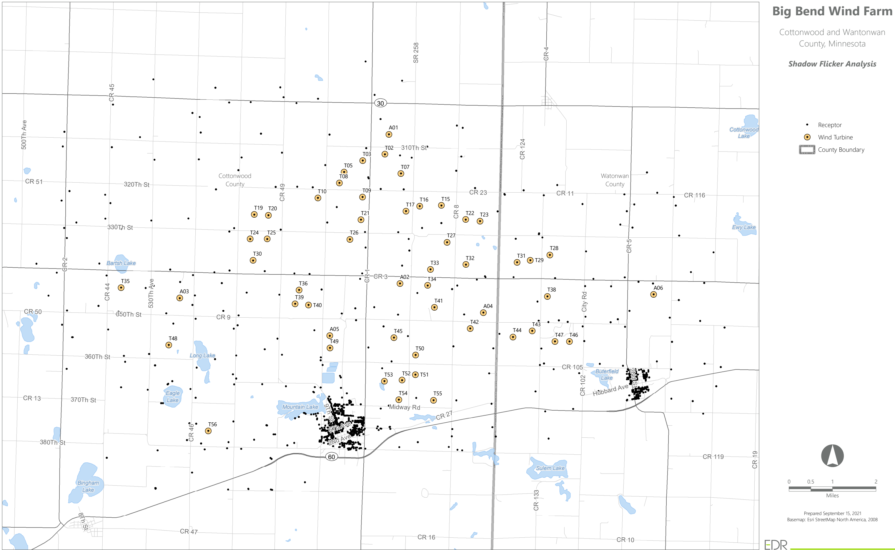
Figure 2. Proposed Turbine Layout
