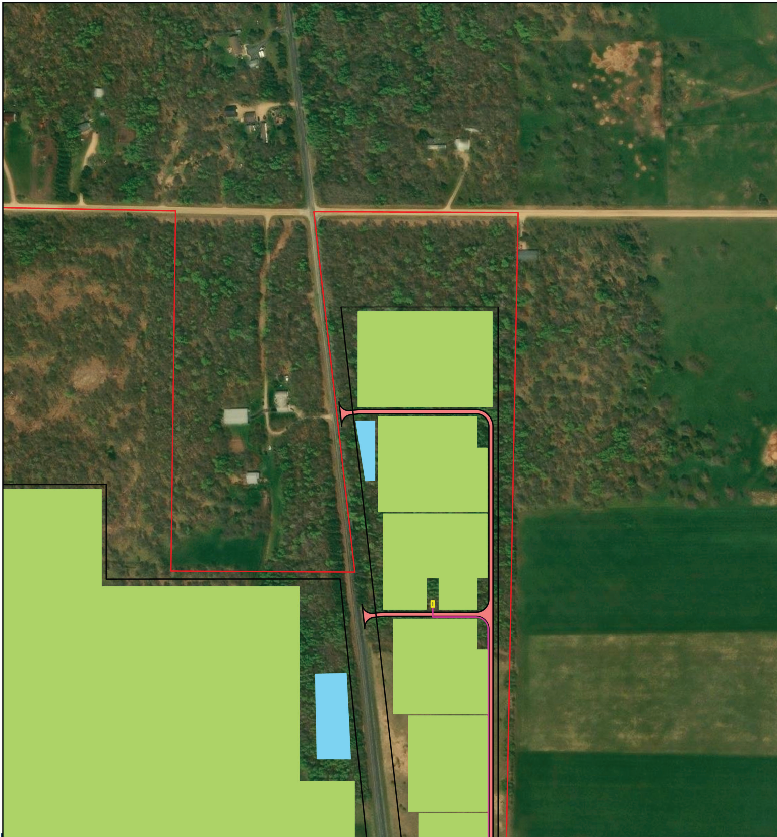
Solway Solar Detail Map | B
