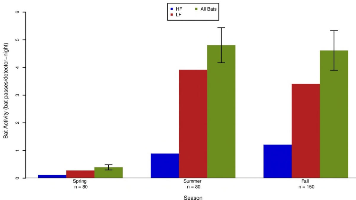
Figure 5a. Seasonal bat activity by high-frequency (HF), low-frequency (LF), and all bats at cropland stations at the Walleye Wind Energy Project from April 14 to October 27, 2016. The bootstrapped standard errors are represented on the 'All Bats' columns.
