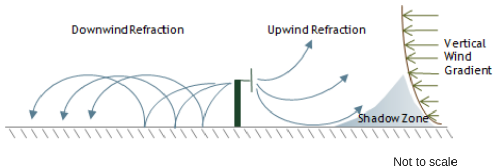
FIGURE 3: SCHEMATIC OF THE REFRACTION OF SOUND DUE TO VERTICAL WIND GRADIENT (WIND SHEAR)
