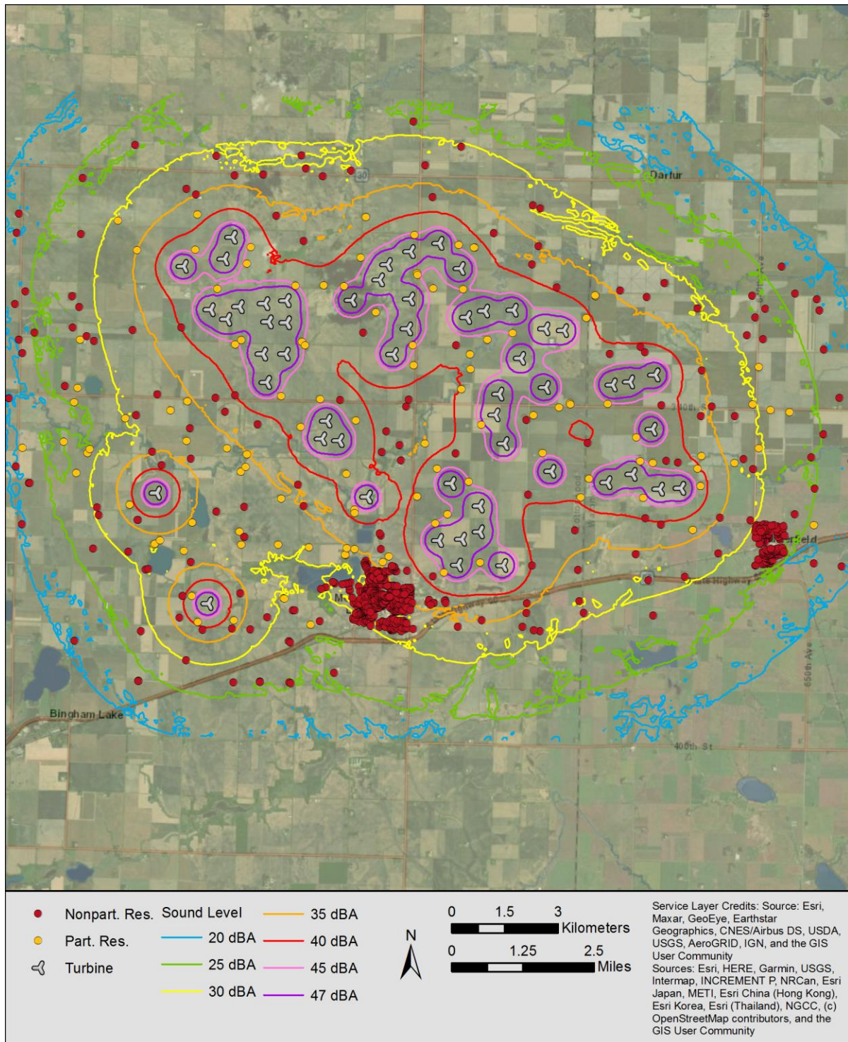
FIGURE 30: SOUND PROPAGATION MODEL RESULTS (TURBINE-ONLY SOUND LEVEL, L_{50} ) NORDEX N163 LNT
