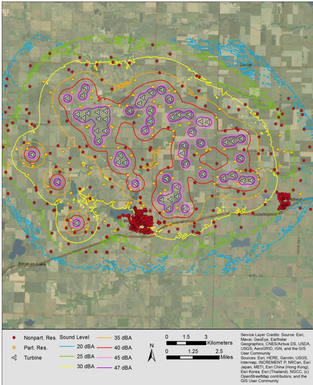
FIGURE 29: SOUND PROPAGATION MODEL RESULTS (TURBINE-ONLY SOUND LEVEL, L_{50} ) GE 5.5-158 LNT E
