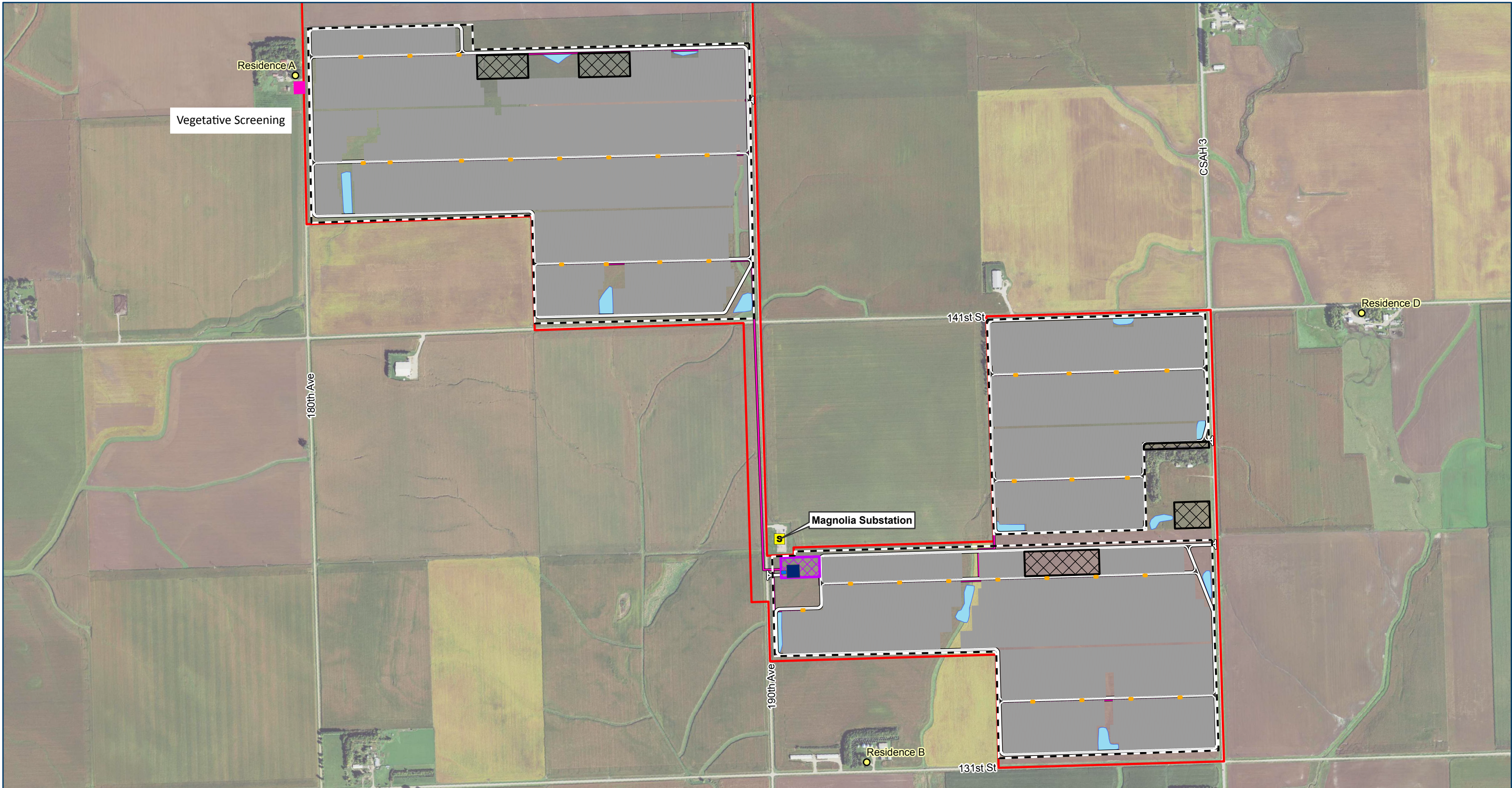
Figure 3: Below Ground Layout
